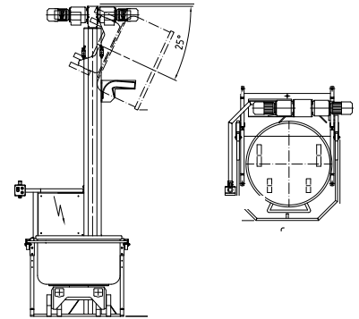
上升和下降及急停均有按钮控制 Push buttons for up/down movements and emergency stop
